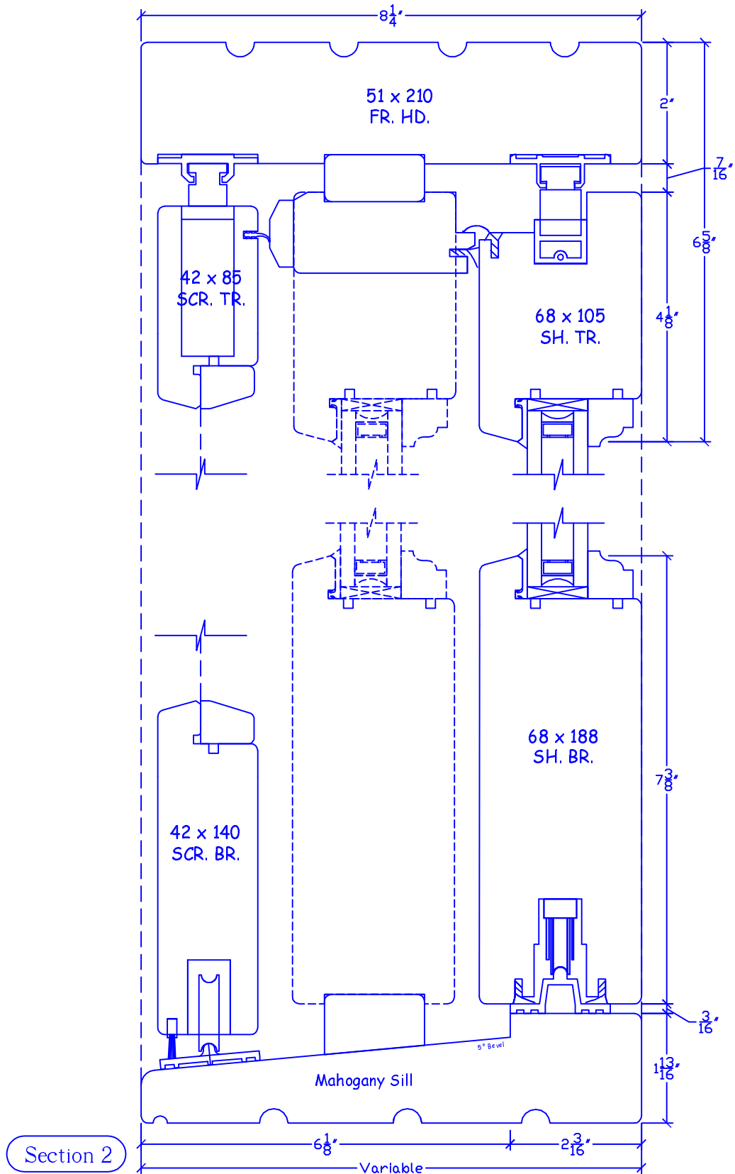
SECTION IN ELEVATION 2-PANEL LIFT-SLIDE DOOR (1 Active, 1 Fixed w/Screen)
