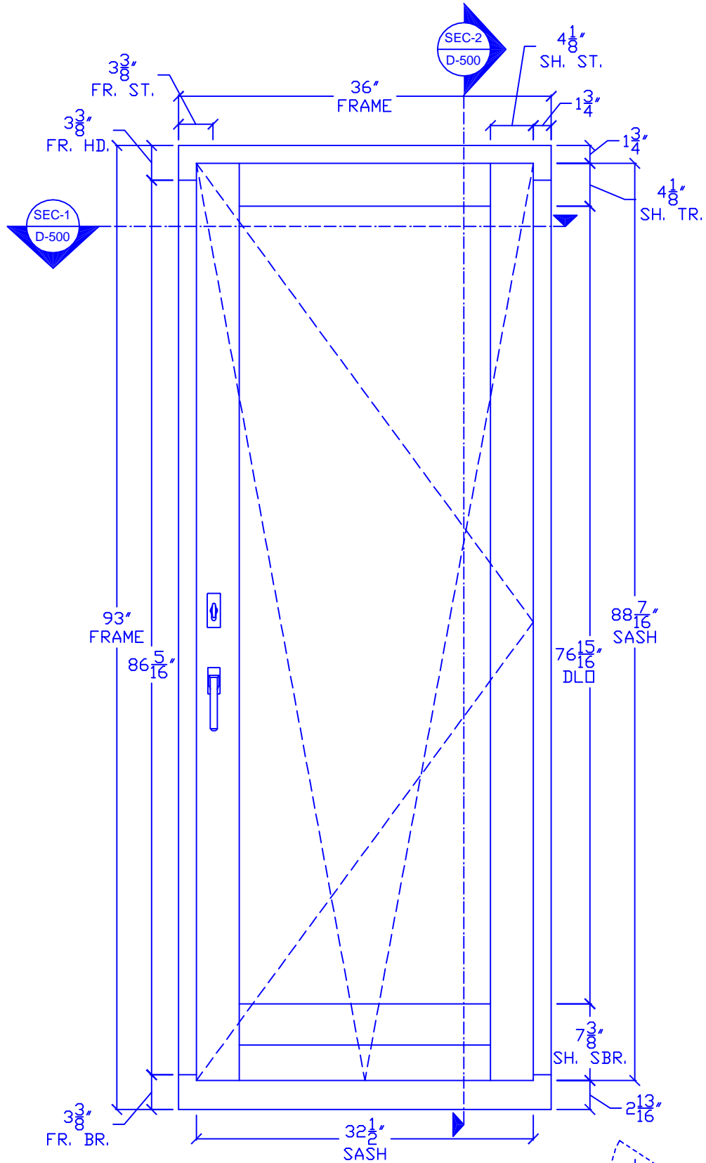
TILT-TURN DOOR UNIT (Single - Stacked Bottom-Rail)
