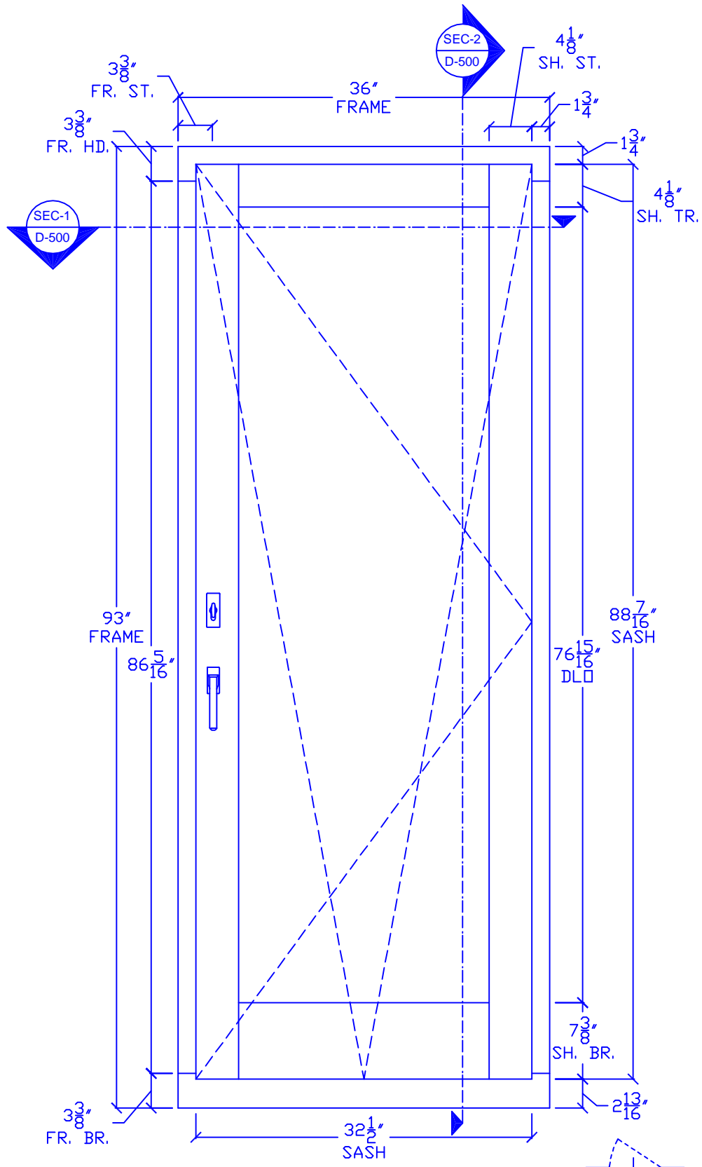
TILT-TURN DOOR UNIT (Single - Solid Bottom-Rail)
