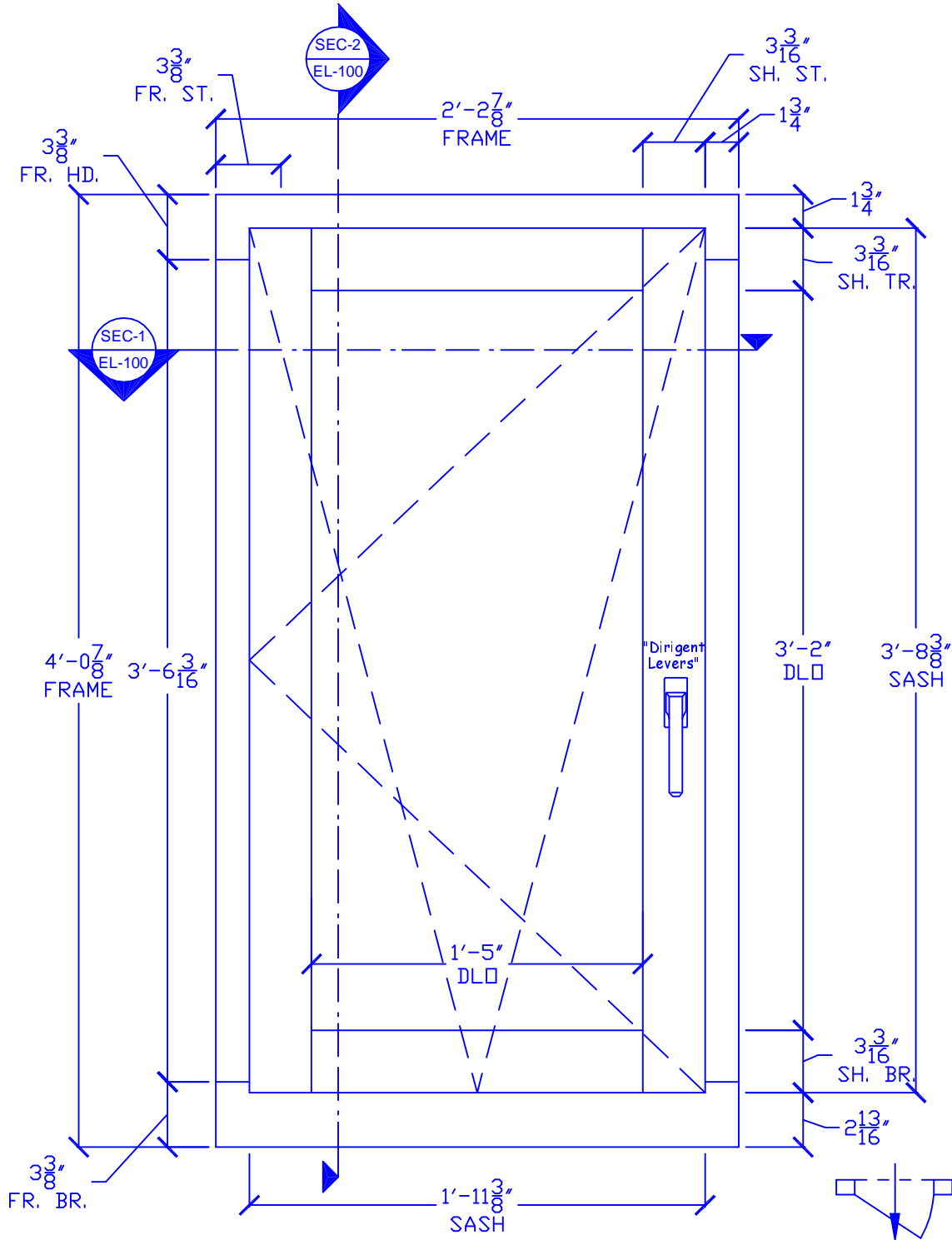
TILT-TURN WINDOW UNIT (Single)
